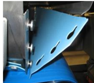
Fig 10. Splashguard with keyhole attachment that can be removed
